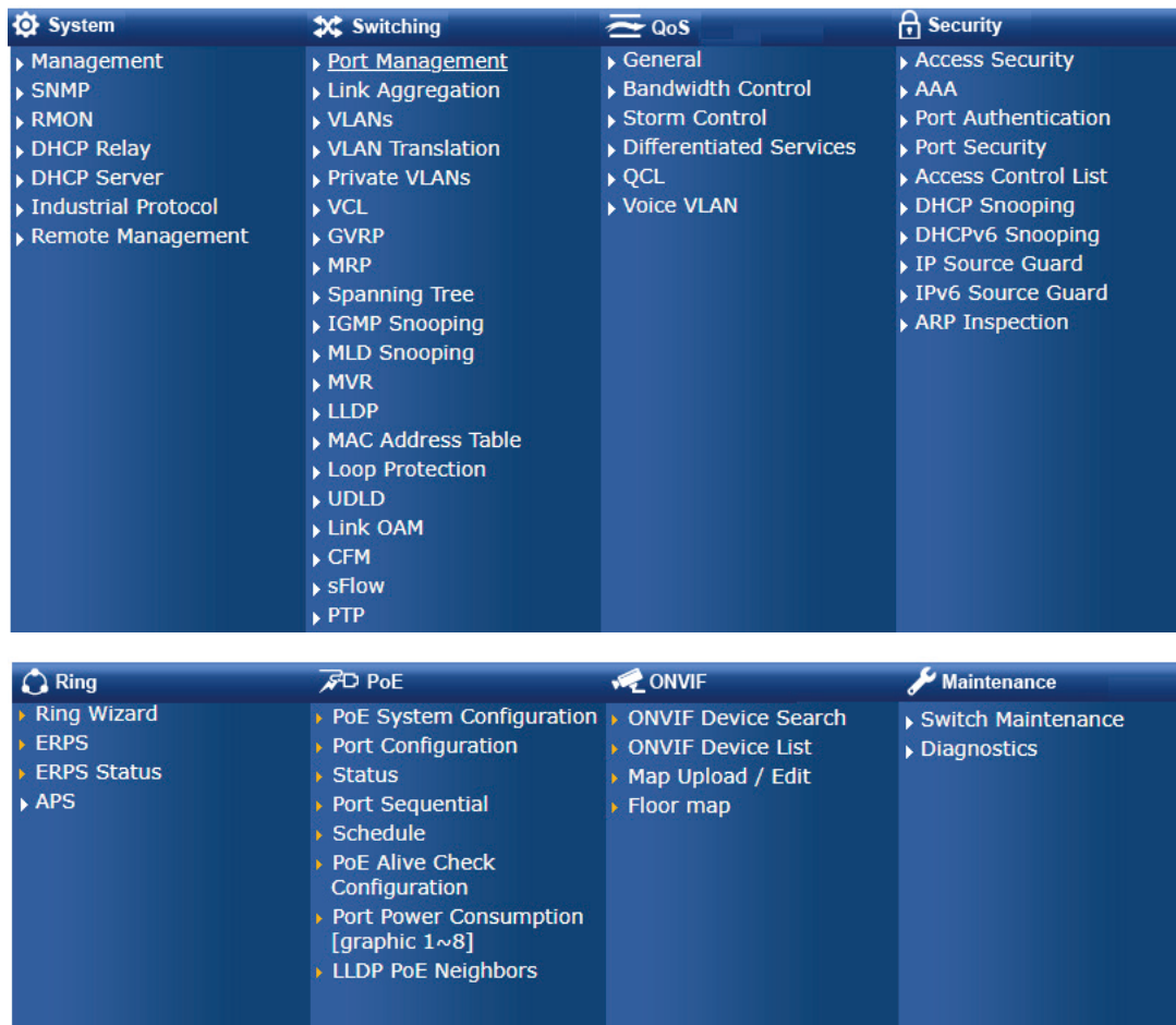
Figure 5-7: Switch Menu
